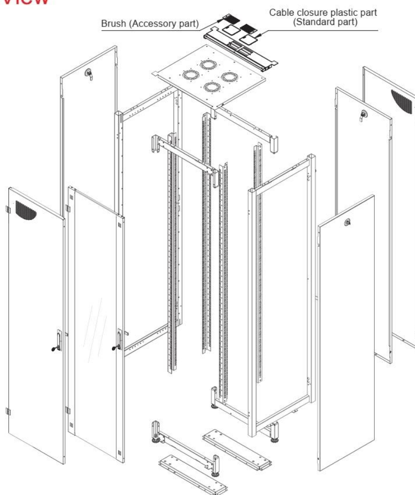
Exploded view
